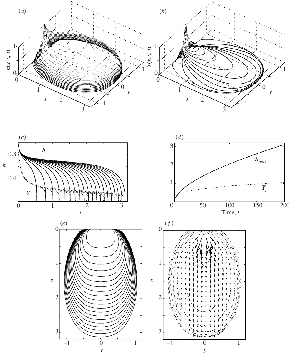
FIGURE 6. Rivulet forming from an outflow from an aperture with B = 1/2 and y_s = 0.1 . (a) The height contours and (b) yield surface at t = 200 (the outermost contour in (b) shows the fluid edge). Also shown are (c) the height profiles (solid and dashed lines) and yield surfaces (dotted lines) along the midsection ( y = 0 ) for times t = 0, 10, 20, \dots, 200 , and (d) the time evolution of the width Y_s (dotted line) and downstream length X_{max} (solid line). (e) A sequence of images of the edge of the fluid taken every 10 time units, and (f) vectors of the depth-averaged velocity field at t = 200 (with superposed height contours).
