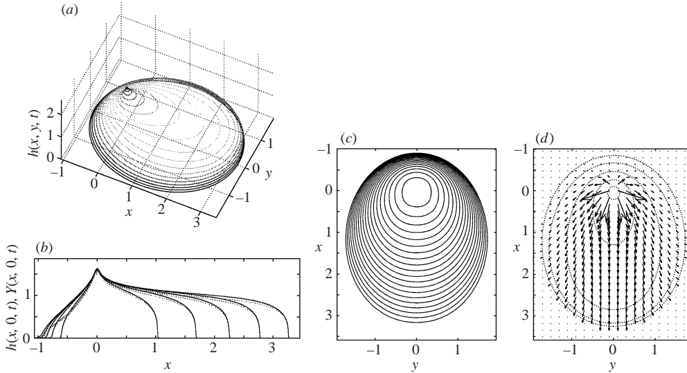
FIGURE 3. A dome with B = 0.067 . (a) A snapshot of the dome at t = 9.4 . (b) Five snapshots of the midsection profile (solid lines) and corresponding yield surface (dotted lines) at times 1.88, 3.76, 5.64, 7.52 and 9.4. (c) A sequence of curves showing the dome's edge (the curves show the edge every 0.38 time units), and (d) vectors of the depth-averaged velocity field at the final time (with superposed contours of constant height).
