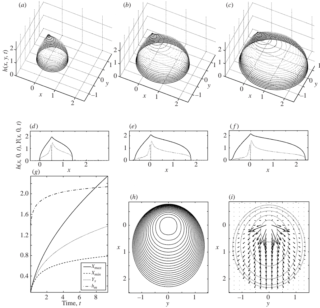
FIGURE 2. An extruded, slumped dome on an inclined plane, computed numerically using the thin-layer model with B = 1.33 . (a–c) Three snapshots of the domes at times 1.88, 5.64 and 9.4, respectively. Directly below, (d–f), are the corresponding height profiles (solid lines) and yield surfaces (dotted lines) along the midsection ( y = 0 ). (g) The evolution of the cross-stream half-thickness ( Y_s ), the downslope and upslope lengths ( X_{max} and X_{min} ), and the maximum height ( h_m ). (h) A sequence of curves showing the dome’s edge (the curves show the edge every 0.38 time units), and (i) vectors indicating the depth-averaged velocity field, h^{-1}(\mathcal{U}, \mathcal{V}) , at t = 9.4 (the dotted curves are contours of constant height).
