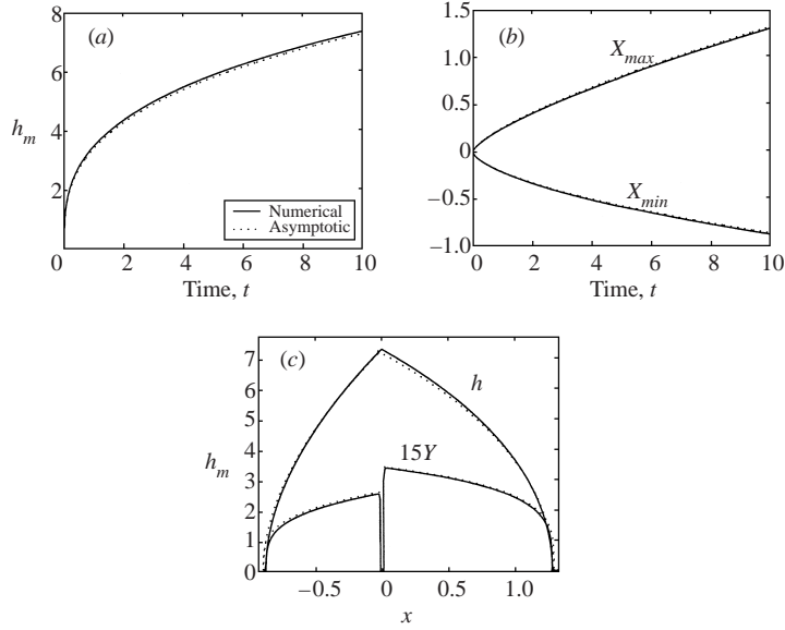
FIGURE 21. Comparison of the numerical and asymptotic solution for n = 1 and B = 25 : (a) maximal height, (b) edge locations, (c) thickness and yield stress. In (c) the comparison is made at t = 10 .
