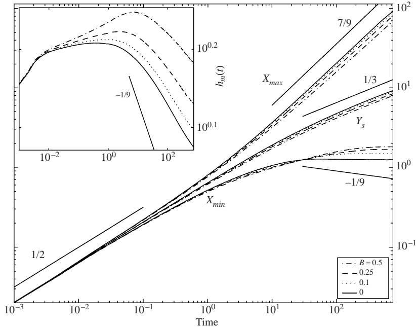
FIGURE 5. Evolution of the dome's characteristic lengths and height for different (but small) values of B and n = 1 . The domain in these computations expands with time. The increase of the domain is determined by the advance of the dome's edges (that is, by approximating X_{min} , X_{max} and Y_s by linear functions of time, and using the corresponding speeds to advance the upper, lower and lateral boundaries of the domain). The vent is fixed in the computational space, and so corresponds to an expanding vent in physical space; the expansion of the vent keeps the ratio of the source radius to dome edge roughly constant, and avoids any gradual loss of resolution at long times. For t < 10^{-2} the linear rise of h_m(t) reflects the initial emplacement of the fluid.
