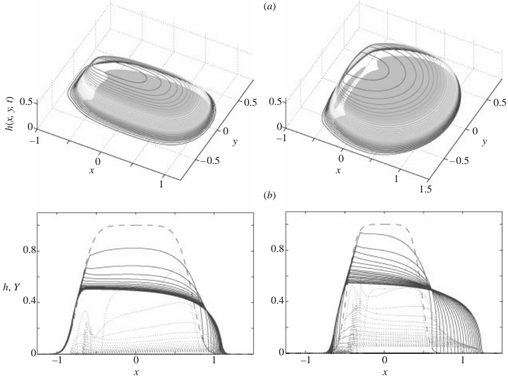
FIGURE 10. Domes created by the slump of a fixed volume. B = 1/2 . (a) The shape of two domes with different initial profiles ((x_*, y_*) = (3/4, 1/4) and (x_*, y_*) = (1/2, 1/2) ) at t = 100 . The shaded region shows the area in which Y > 0 . (b) The corresponding height profiles (solid and dashed lines) and yield surfaces (dotted lines) along the midsection ( y = 0 ) for times t = j^2/4 with j = 0, 1, 2, \dots, 20 .
