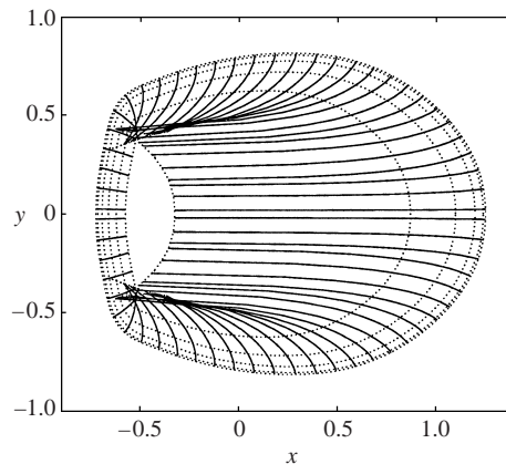
FIGURE 16. The characteristics solution for the slumped dome corresponding to the computation shown on the right of figure 10, with B = 1/2 and (x_*, y_*) = (1/2, 1/2) . The solution is constructed using the dome edge at the end of the computation, and assumes that the structure yielded everywhere during the slump and has come to rest, neither of which is quite correct. However, the picture illustrates only how the characteristics cross. The characteristics are drawn only up to a certain height less than the maximal value for the sake of clarity (the crossings of the characteristics otherwise makes the picture unreadable).
