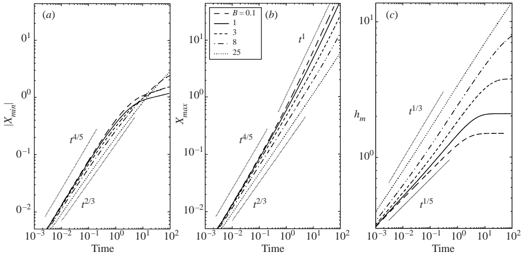
FIGURE 20. Evolution of (a) upstream length, (b) downstream length and (c) maximum height for extrusions with varying B . For these computations, in order to better resolve the solution, the domain of the computation was split into upstream and downstream sections that moved approximately with the fluid edges, and the source function was replaced by a boundary condition at x = 0 .
