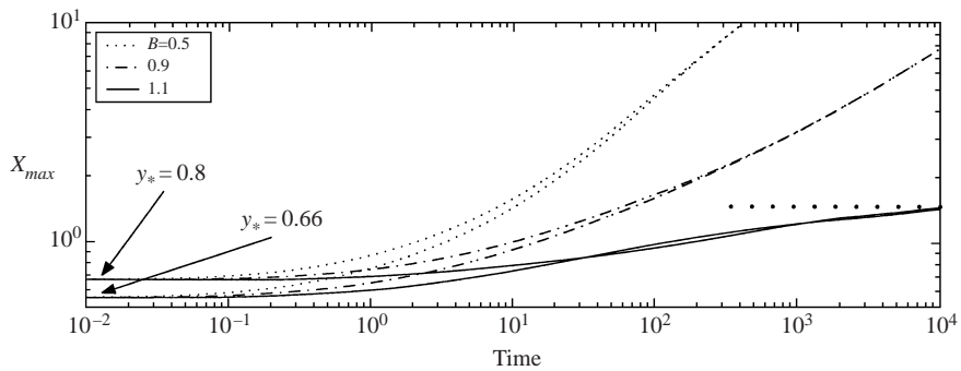
FIGURE 9. The progression of the downslope length, X_{max} , with time for several rivulets with varying B and y_* . The dots display the expected limiting value for B = 1.1 , which is given by SX_{max} = (B/S) \log[B/(B - S)] - 1 \approx 1.64 (with S = 1 ).
