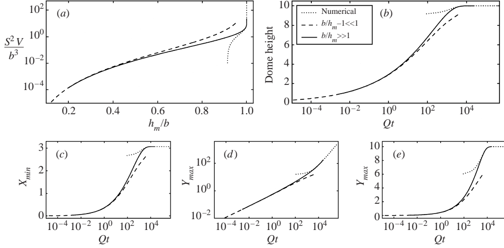
FIGURE 12. (a) S^2V/b^3 as a function of h_m/b = Sh_m/B , computed by evaluating the quadrature in (4.11) numerically. For b \gg h_m , S^2V/b^3 \sim 2\pi h_m^3/(15\psi^3 b^2) , where \psi^2 = b^2/h_m^2 - 1 , whilst for b/h_m - 1 \ll 1 , S^2V/b^3 \sim \pi h_m^3 [\log(2/\psi) - 3/2]/b^2 . These two limits are also included in the figure. Given the function shown in (a), we may construct sample extrusions in the large- B limit given specific values of S and B . This is done in the other panels of the figure for B = 10 , S = 1 : (b) dome height, (c) upstream length, (d) downstream length, (e) width. Again, the two limiting forms of V are added in (c–e).
