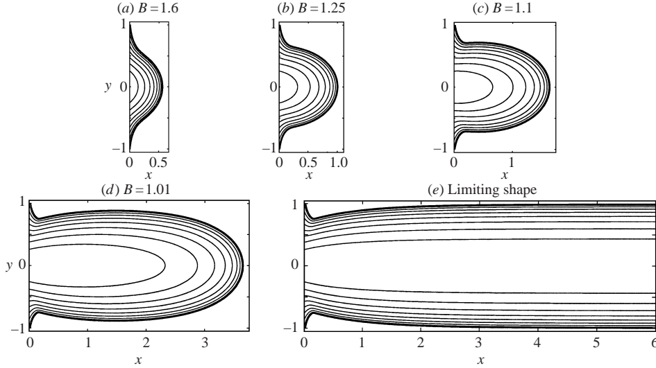
FIGURE 14. Contours of constant height (spaced by 0.1) for stationary rivulets emerged from a Gaussian orifice with half-width y_* = 0.8 . Shown are four values of B , and the limiting shape as B \rightarrow 1 (with S = 1 ).
