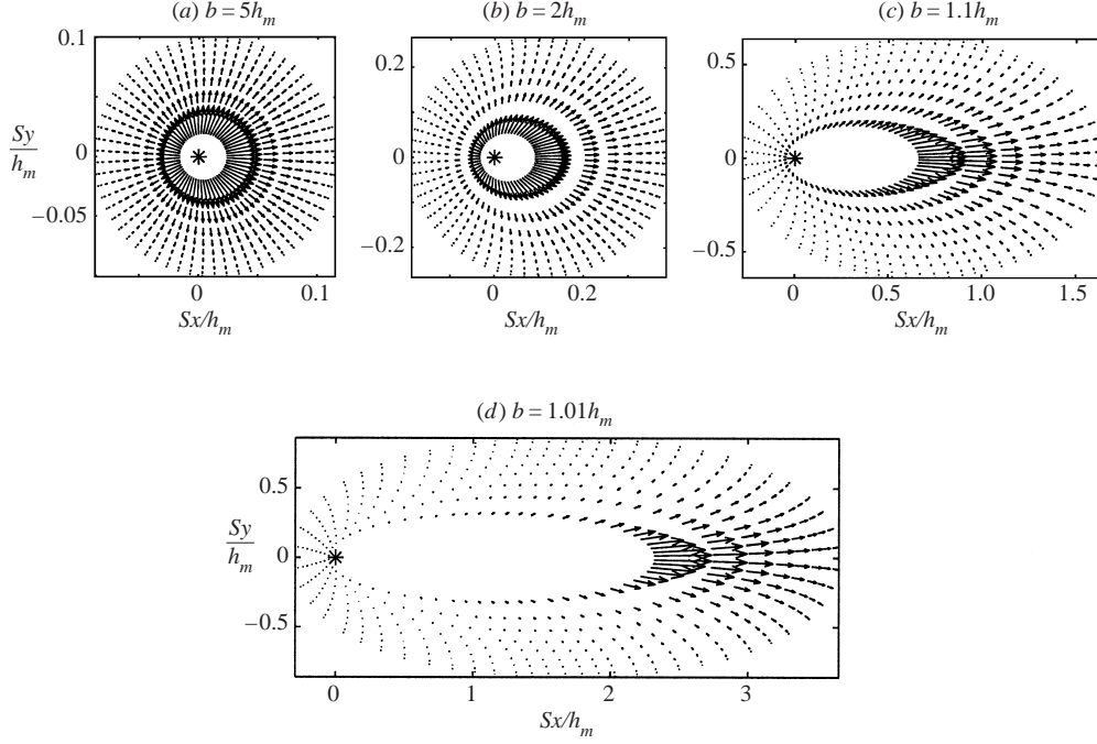
FIGURE 13. Pattern of the depth-averaged velocity field for the domes shown in figure 11(a–d).
