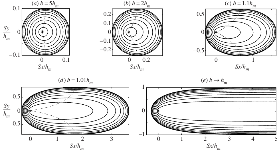
FIGURE 11. Contours of constant height (spaced by h_m/10 ) for yield-stress-dominated domes on sloping planes. The dotted curves show the a = 0 characteristic that connects to the widest part of the dome ( a-d ). Contours of constant height for the limiting shape as b \rightarrow h_m ( e ).
