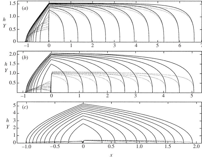
FIGURE 19. The thickness and yield surfaces for constant extrusion from a line source with (a) B = 0.1 , (b) B = 1 and (c) B = 10 (and n = 1 ). The solutions are shown at unit intervals in t .
