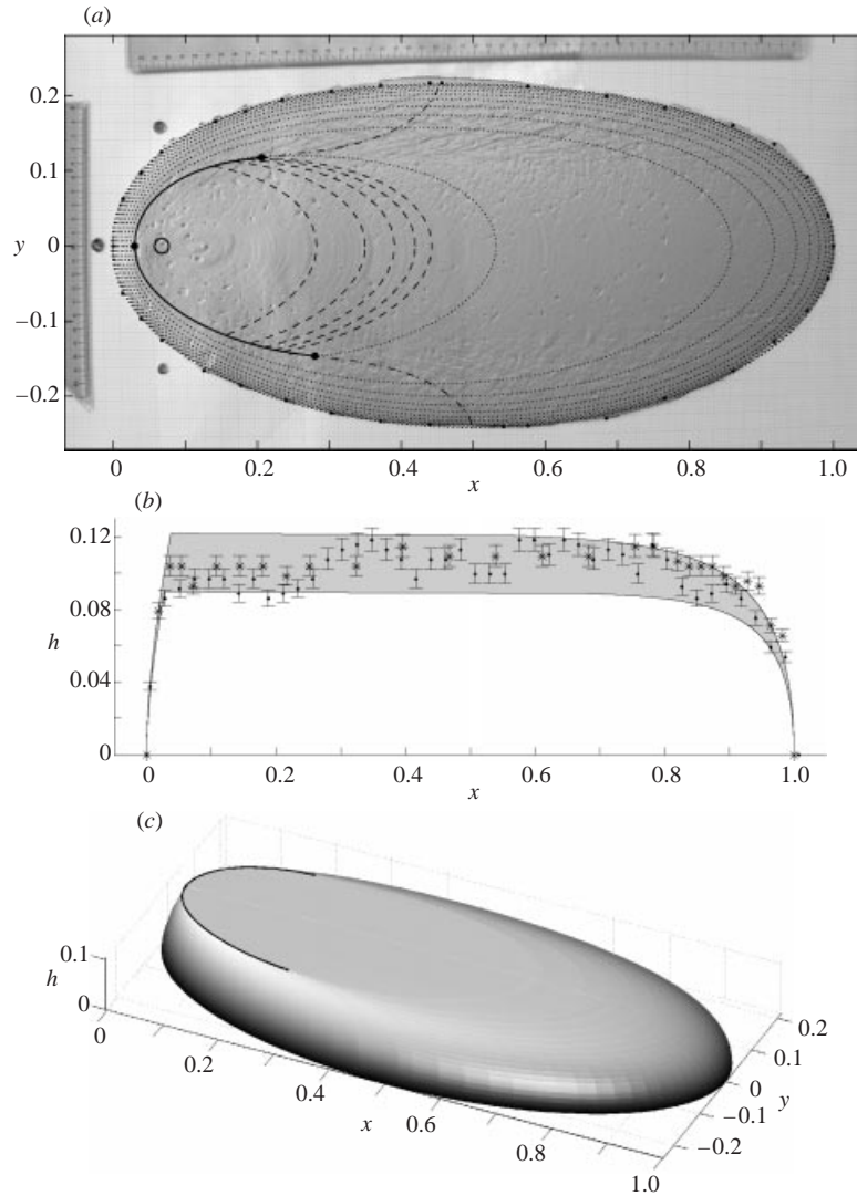
FIGURE 17. Comparison between the theory and an experiment in which we spilled a fixed volume (about 11) of a kaolin-based slurry onto an inclined plane. The slurry was formed by diluting ‘joint compound’ (Sheetrock Brand, United States Gypsum Company) with water (in the ratio of 7.5 kg of compound to 11 kg of water). (a) Theoretical contours of constant thickness superposed onto a photograph from the experiment. The dotted contour levels are spaced by 0.01, whilst the dashed contours near the maximal height are spaced by 4 \times 10^{-5} . The dashed-dotted line shows the characteristic along which the seam first occurs, and the solid curve delimited by dots is the seam. The dot midway along the seam is the position of maximum height. (b) The theoretical and experimental midsection profiles. The characteristics solution is constructed from the observed fluid edge (fit with the function y^2 = f(x) , where f(x) is a quartic polynomial); the full solution, with its seam, is shown in (c). The lengths and thickness are shown in dimensionless units obtained using the total slopewise length of the deposit, and S = 1 (which fixes H = L \tan \phi and not to be the maximum thickness). The slope angle is \phi \approx 9.5^\circ , and the slurry is spilled into the localized region indicated by the circle in (a). The yield stress, \tau_p \approx 22 Pa s, was estimated by spilling the slurry onto a horizontal plane (cf. Osmond & Griffiths), and using the formula, \tau_p = \rho g (\text{height})^2 / (\text{diameter}) ( \rho \approx 1440 kg m ^{-3} ). From \tau_p , L and \phi , we estimate that B = \tau_p / (\rho g L^2 \sin \phi) \approx 0.1 . Two sets of independent measurements of thickness are shown in (b), and the spread of points gives some idea of the measurement error. The vertical error bars and the shaded theoretical band indicate the uncertainties stemming from the non-dimensionalization of h (that is, H ) and contained in B .
