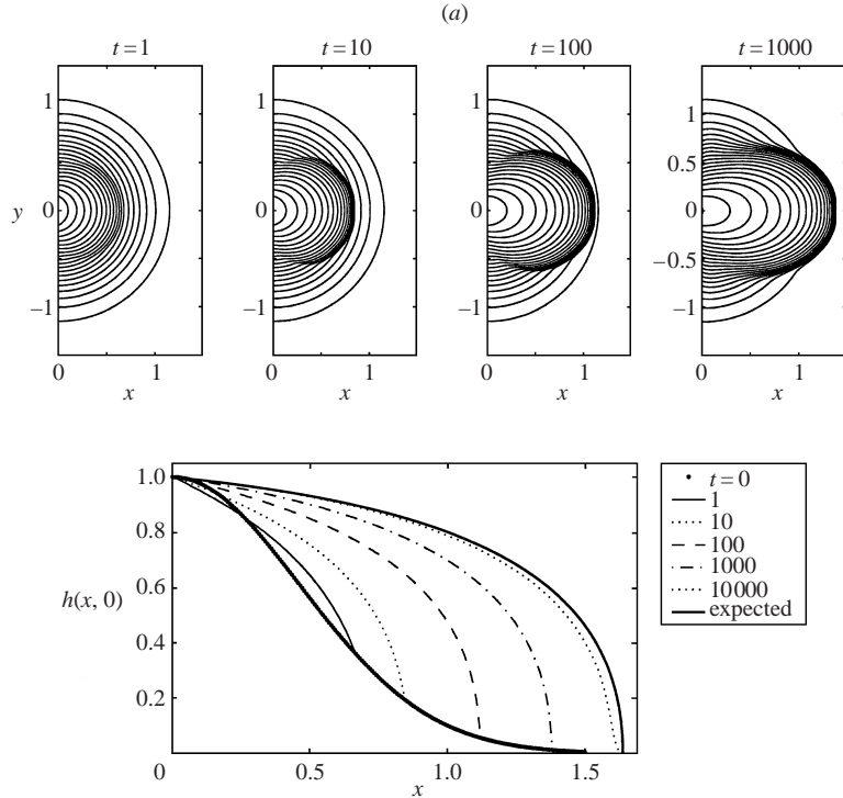
FIGURE 8. (a) Four snapshots of a rivulet spreading out from an aperture with y_* = 0.66 . B = 1.1 . Contour levels begin at h = 0.1 and then increase to unity in steps of 0.05. (b) Five snapshots of the midsection. The initial condition is also shown, as is the expected final profile based on the theory of §4.2, given by (3.12).
