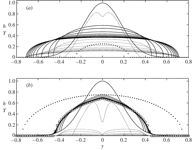
FIGURE 18. The thickness (solid lines) and yield surfaces (dotted lines) for spreading uniform rivulets with (a) B = 1/4 and (b) B = 3/4 . The initial profile has a characteristic half-width of y_* = 0.25 . The dots show the maximum stationary profile at that yield stress; the circles in (b) show the approximate final shape. The solutions are shown at intervals of 1.25 in t .
