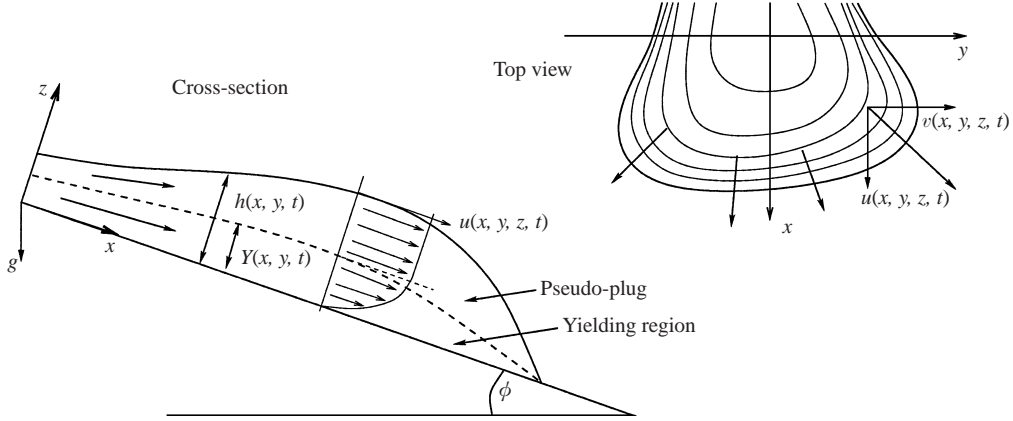
FIGURE 1. Sketch of a flow on an inclined plane. \phi is the angle of inclination to the horizontal, z is perpendicular to the plane, x is directed downslope, and y is the cross-slope coordinate.
