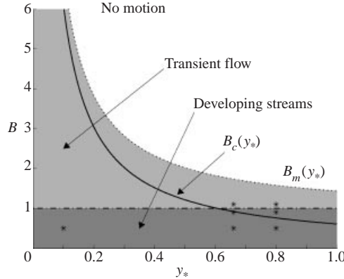
FIGURE 7. Regime diagram on the (y_*, B) -plane for rivulets with the initial and y = 0 boundary condition, h(x, y, 0) = \exp[-(x^2 + y^2)/y_*^2] . B_m(y_*) is the maximum value of sh at t = 0 (the greatest initial gravitational stress); if B > B_m(y_*) , the initial profile is held in position by the yield stress. The horizontal line, B = Sh_{max} \equiv 1 , marks the limit below which rivulets expand inexorably into flowing streams. The two lines, B = B_m(y_*) and B = 1 , divide the parameter plane into three characteristic regimes (no motion, transient flows, developing streams). The curve B_c(y_*) is the boundary below which the characteristics solution of §4.2 is not valid. The stars locate the parameter settings used in the computations.
