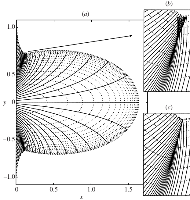
FIGURE 15. The characteristics solution for a rivulet emerging from a Gaussian aperture with B = 1.1 and y_* = 0.66 . The region over which the characteristics cross is shown in more detail in (b). Panel (c) shows the single-valued surface that we construct by inserting a ‘seam’ into the solution according to the argument given in the main text.
