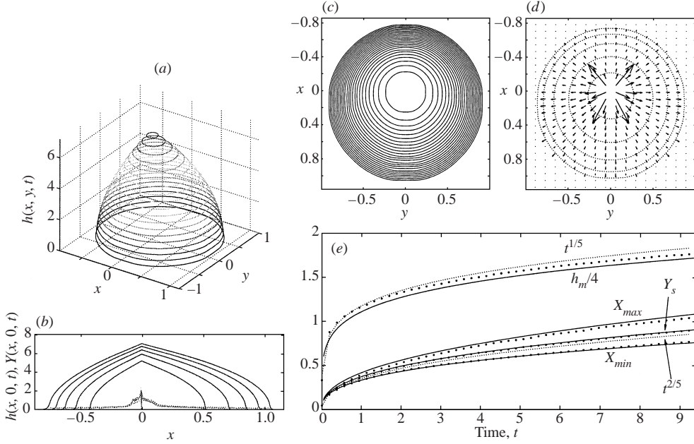
FIGURE 4. A similar picture to figure 3, but for a dome with B = 26.6 . The additional picture (e) shows the height (divided by four, for clarity) and the characteristic lengths. The points show the numerical computations and the solid lines indicate the analogous results for the large- B theory of §4. The dotted lines show the characteristic scalings, t^{1/5} and t^{2/5} .
